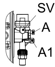
Ansicht HG(X)4/555 -4 (S) R134a View HG(X)4/555 -4 (S) R134a
